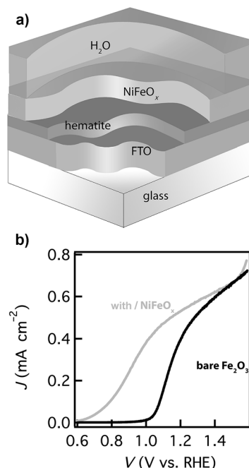
Figure 1. Effect of surface modification with a \text{NiFeO}_x overlayer on the PEC performance of hematite. a) Schematic perspective view of the modification. b) Photocurrent-density–voltage plot showing the substantial cathodic shift (up to 0.38 V) observed upon the surface modification of hematite with \text{NiFeO}_x . FTO = fluorine-doped tin oxide.
